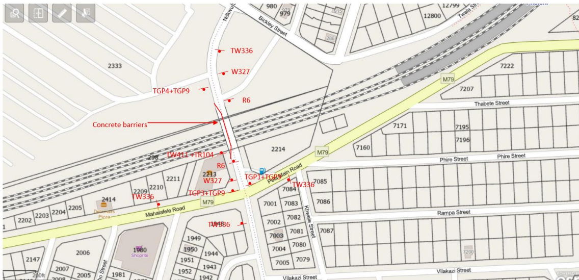
Above: Temporary lane closure and traffic deviation plan
